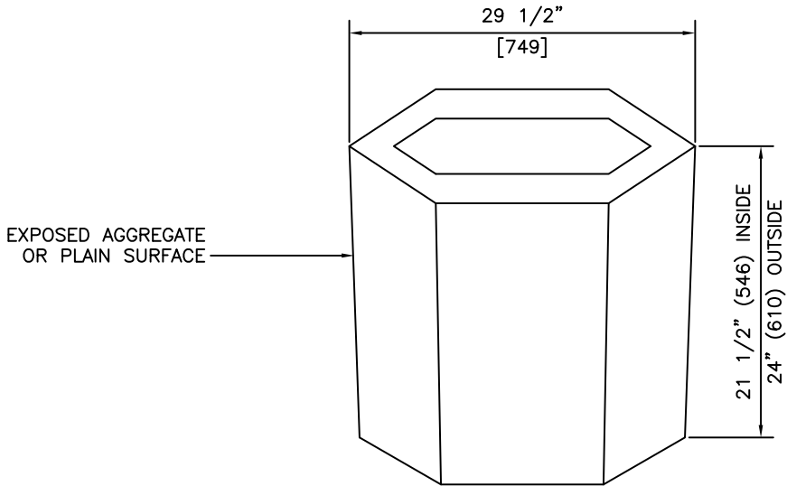
ISOMETRIC
